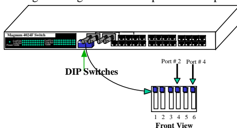
Fig 3.5 Dip Switch Settings
