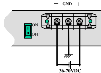
Figure B4.1: -48VDC Terminal Block on Magnum Ks-48VDC
